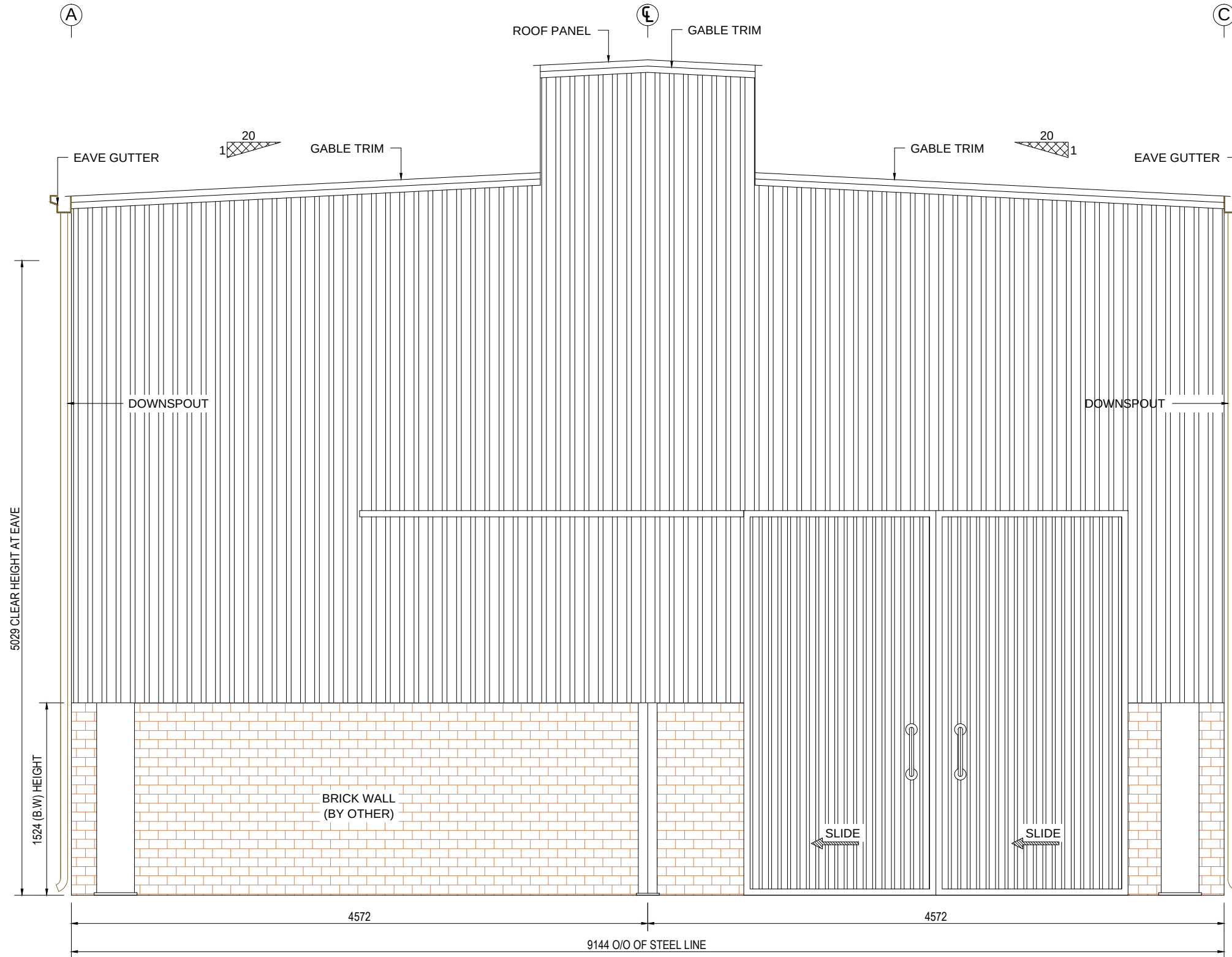
END WALL SHEETING @ GRID-1
